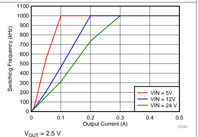
Figure 18. Auto PFM Mode Switching Frequency vs Output Current
