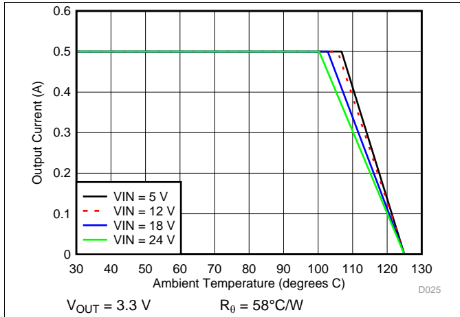
Figure 13. Ambient Temperature vs Output Current
