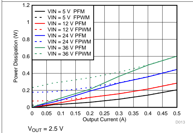
Figure 15. Power Dissipation
