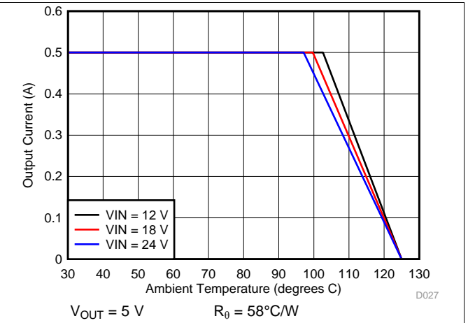
Figure 14. Ambient Temperature vs Output Current
