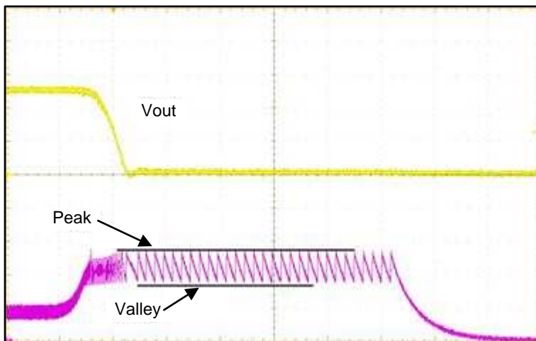
Figure 27. Current Limit Operation During Output Short Circuit
